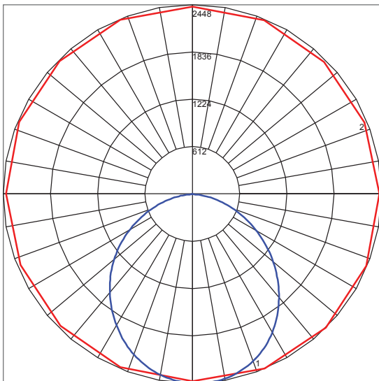
Maximum Candela = 2447.76 Located At Horizontal Angle = 315, Vertical Angle = 3 # 1 - Vertical Plane Through Horizontal Angles (315 - 135) (Through Max. Cd.) # 2 - Horizontal Cone Through Vertical Angle (3) (Through Max. Cd.)
