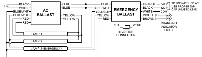
FIG F THREE (3) LAMP RAPID START BALLAST
