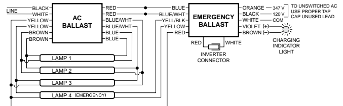
FIG H FOUR (4) LAMP RAPID START BALLAST
