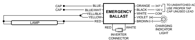
FIG I ONE (1) 17-40 W LAMP WITHOUT AC BALLAST
