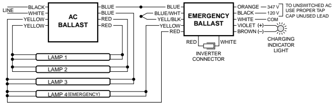
FIG G FOUR (4) LAMP INSTANT START BALLAST
