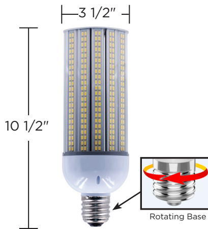
LCE39-40C-T3 Type 3 LED Lamp 40 Watt, 4000K, 5600lm Replaces up to 250W MH 180° Adjustable Beam Angle DLC Listed lamp #GKS13-40W-06D3
