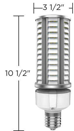
LCE39-54C-DS Dark Sky LED Lamp 54 Watt, 4000K, 5900lm Replaces up to 250W MH 180° Down Beam Angle DLC Listed lamp #GKS28-54W Plus(4000K)
