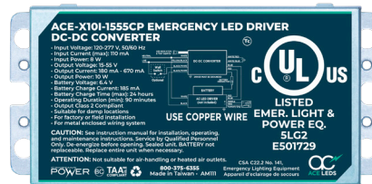
DC-DC CONVERTER
