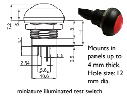
miniature illuminated test switch
