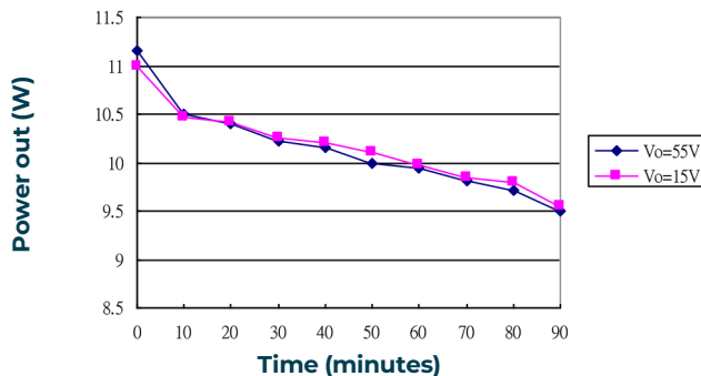
Constant output power performance over full 90 minutes run-time
